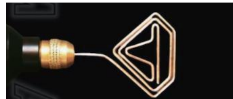
Warm Plasma
