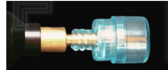
Warm Plasma
